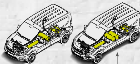
CARGO MAXI VERSION WITH ADDITIONAL METHANE TANK (OPT. 422)
